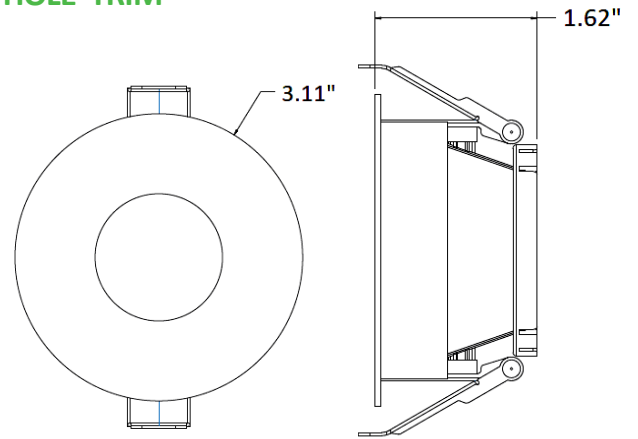
Pin Hole Trim Dimension
